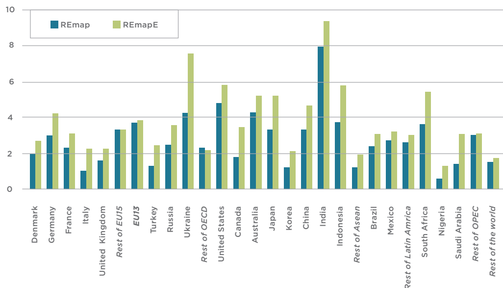
Figure 3: National welfare impacts of doubling renewable energies by 2030, with and without increased power generation (IRENA, 2016)
